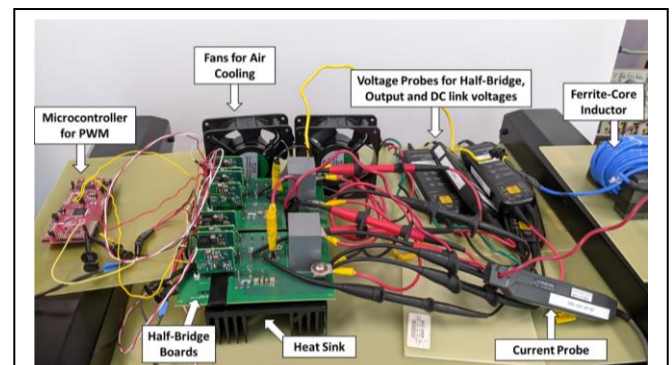
Fig. 16. The BiDFET H-bridge assembly being operated as a Voltage-Source Inverter with an R-L load.
