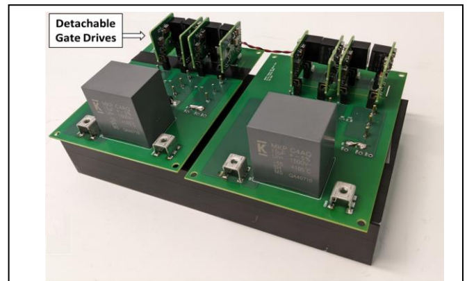
Fig. 15. A H-bridge assembly made using two SSC HB BiDFET modules connected in parallel.
